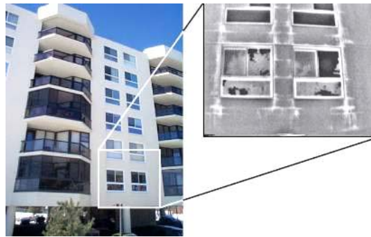
Thermographic image depicting water intrusion around windows.
