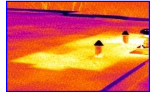
Thermographic image of moisture in roofing
